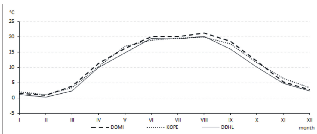
Fig. 2: Average soil temperatures at selected MESSO stations, 2011
