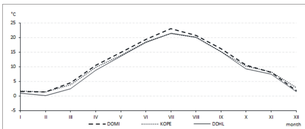
Fig. 1: Average soil temperatures at selected MESSO stations, 2010
