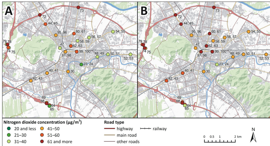
Fig. 8: Concentrations of nitrogen dioxide in open space along roads in the summer (A) and winter (B) measuring campaigns. Sources: GURS, 2012 and MKGP, 2013 for GIS data; authors' survey for NO 2 concentrations
