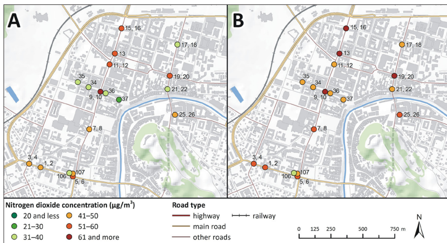
Fig. 9: Concentrations of nitrogen dioxide in street canyons in the summer (A) and winter (B) measuring campaigns. Sources: GURS, 2012 and MKGP, 2013 for GIS data; authors' survey for NO 2 concentrations
